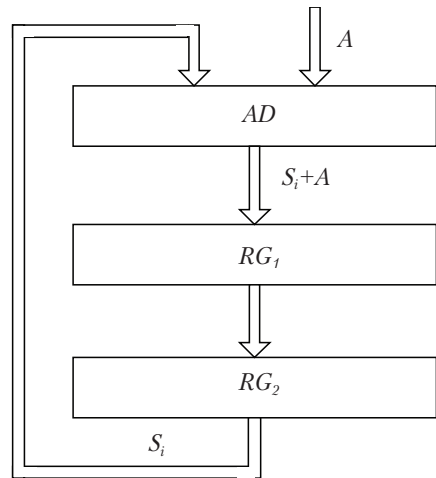
Figure 10.12. Mirror-symmetric accumulator
