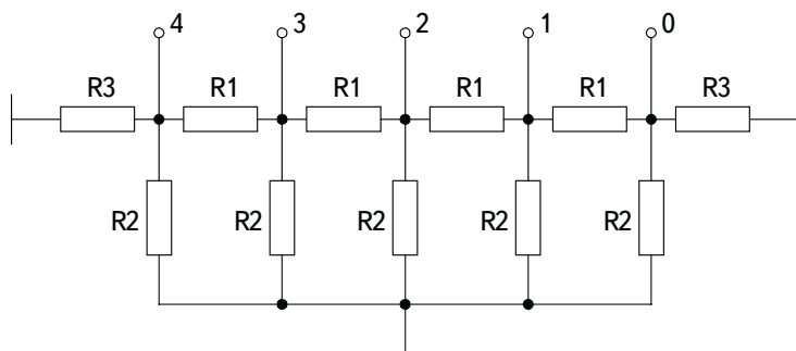
Figure 9.1. Resistor dividers
