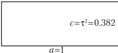
Figure 1.7. The Euclidean rectangle
