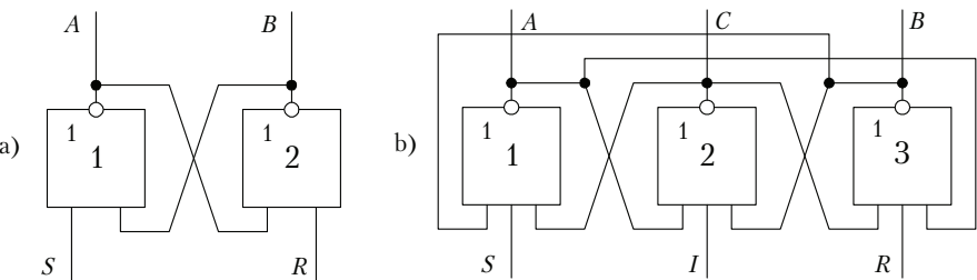
Figure 10.5. “Flip-flop” (a) and “flip-flap-flop” (b)
